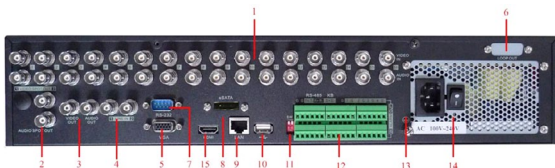
Rear Panel of DS-9116HFI-RH
